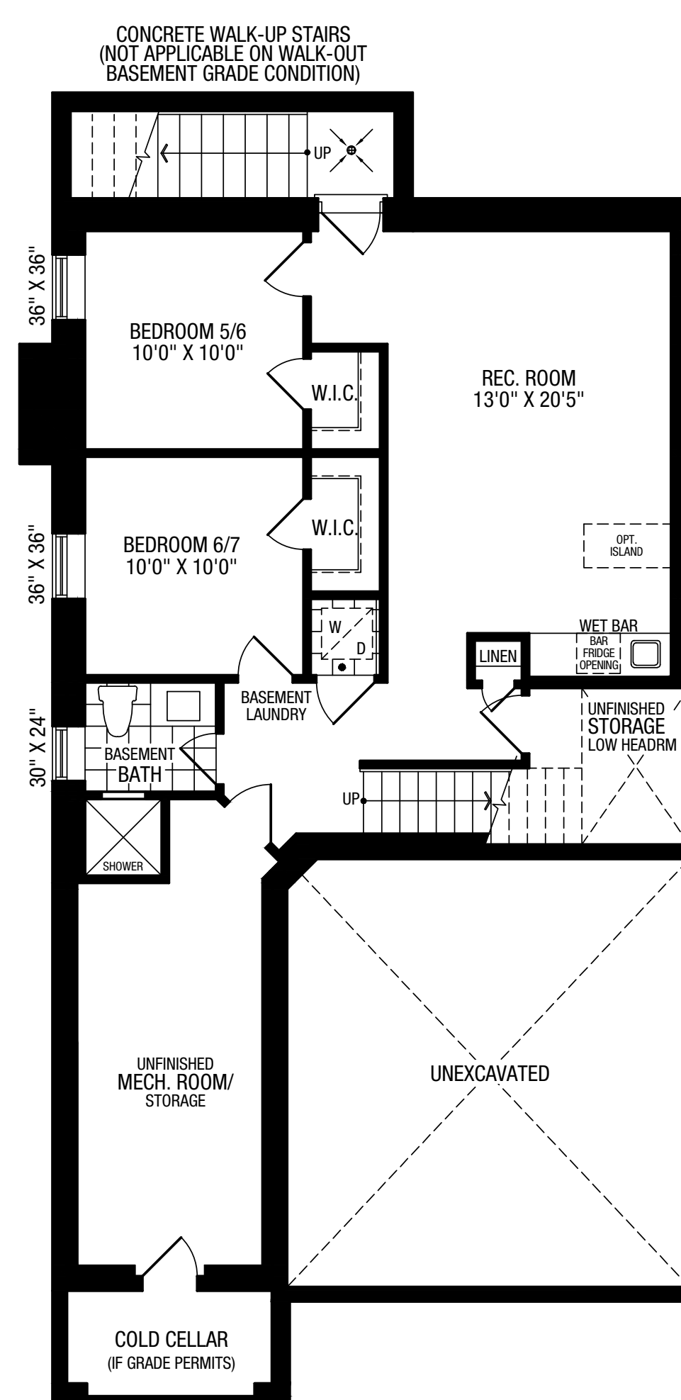
STANDARD FINISHED 740 SQ. FT.
