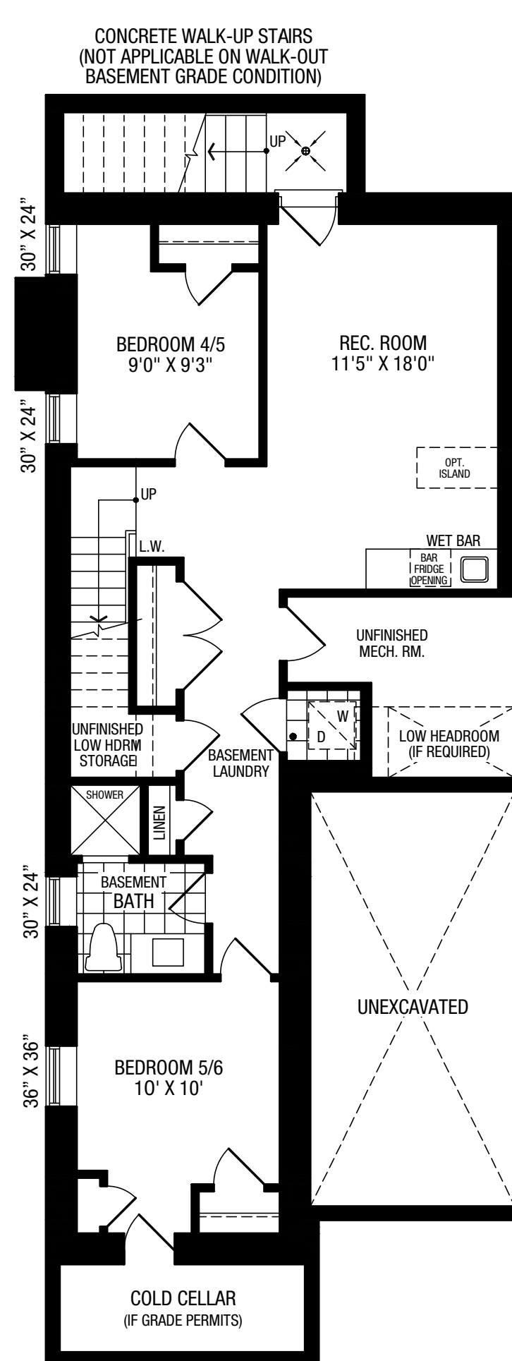
STANDARD FINISHED 739 SQ. FT.
