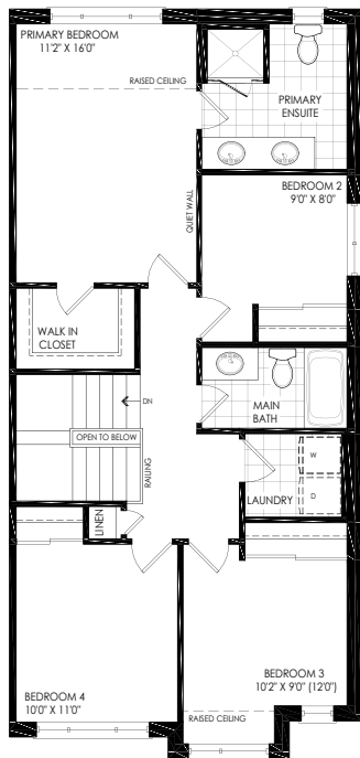
UPPER FLOOR 'STYLE 'A1'
