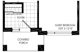
PARTIAL LOWER FLOOR STYLE 'A2'
